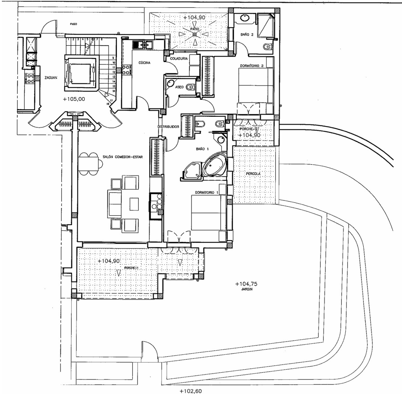
Plano BRR1
