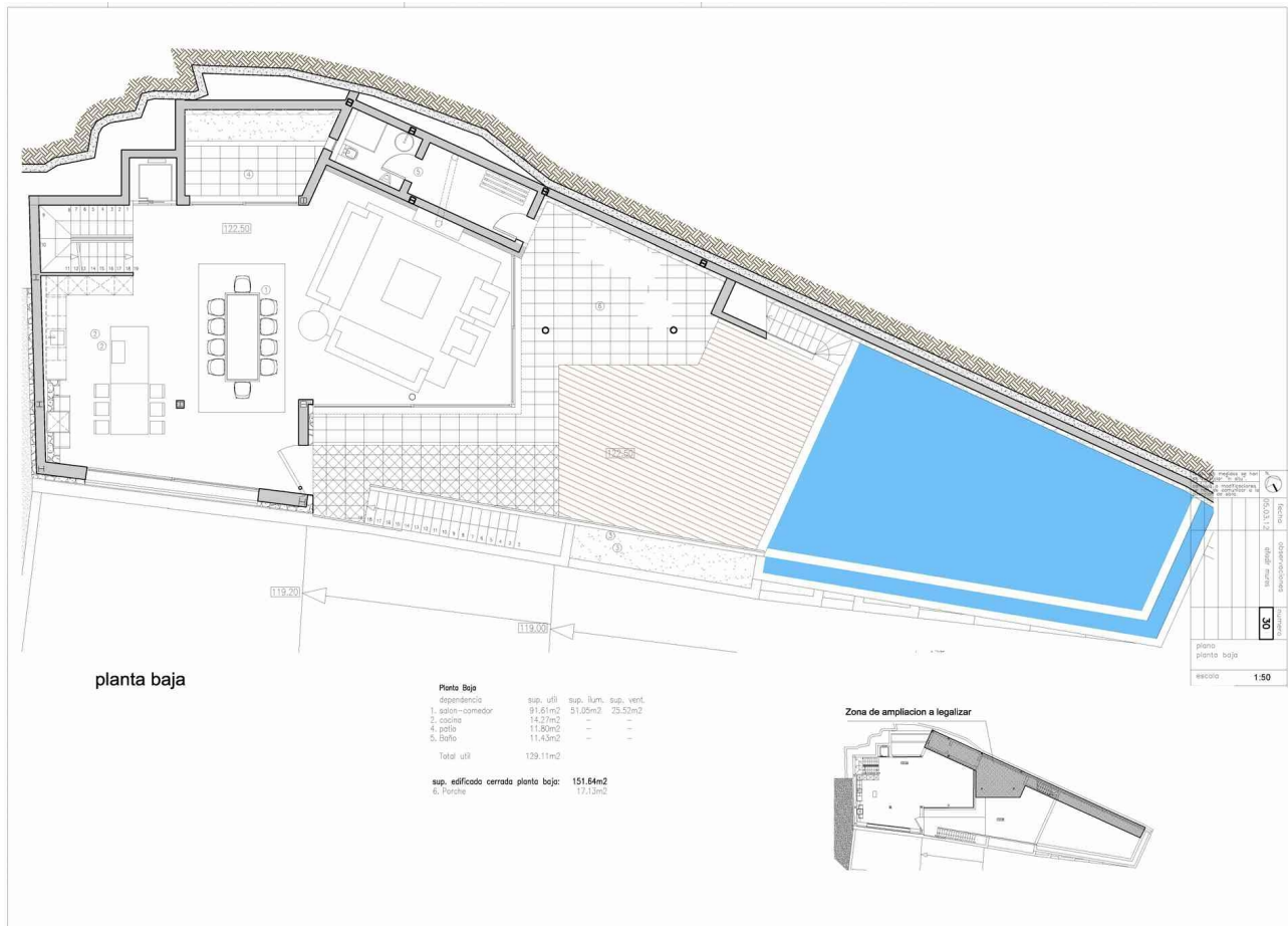
Floorplan Groundfloor
