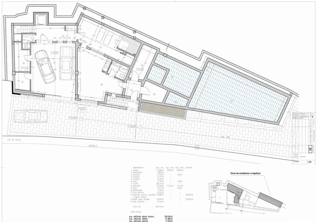
Floorplan Basement
