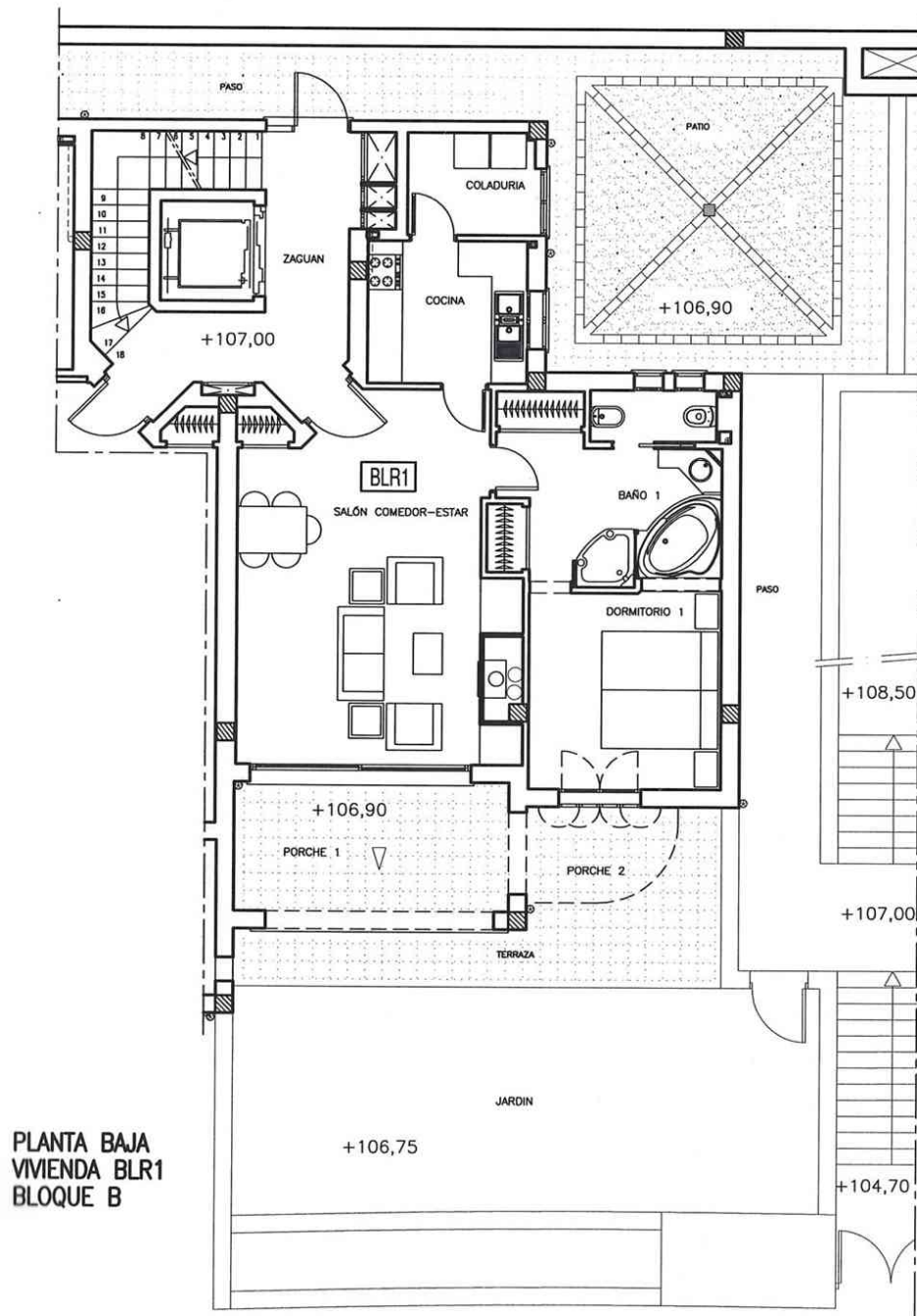
Floorplan
