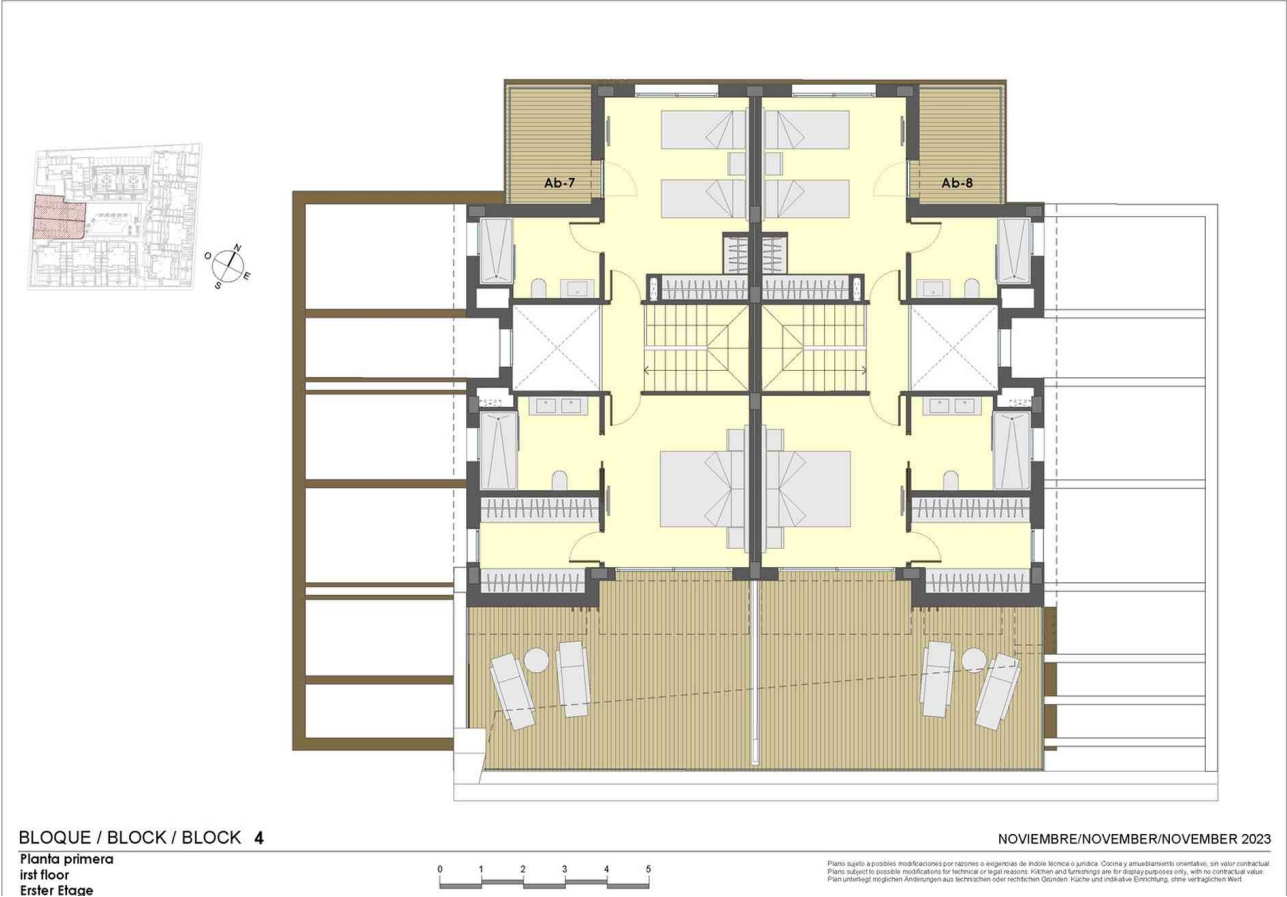
FFloorplan Villa 07 (Upper Floor)
