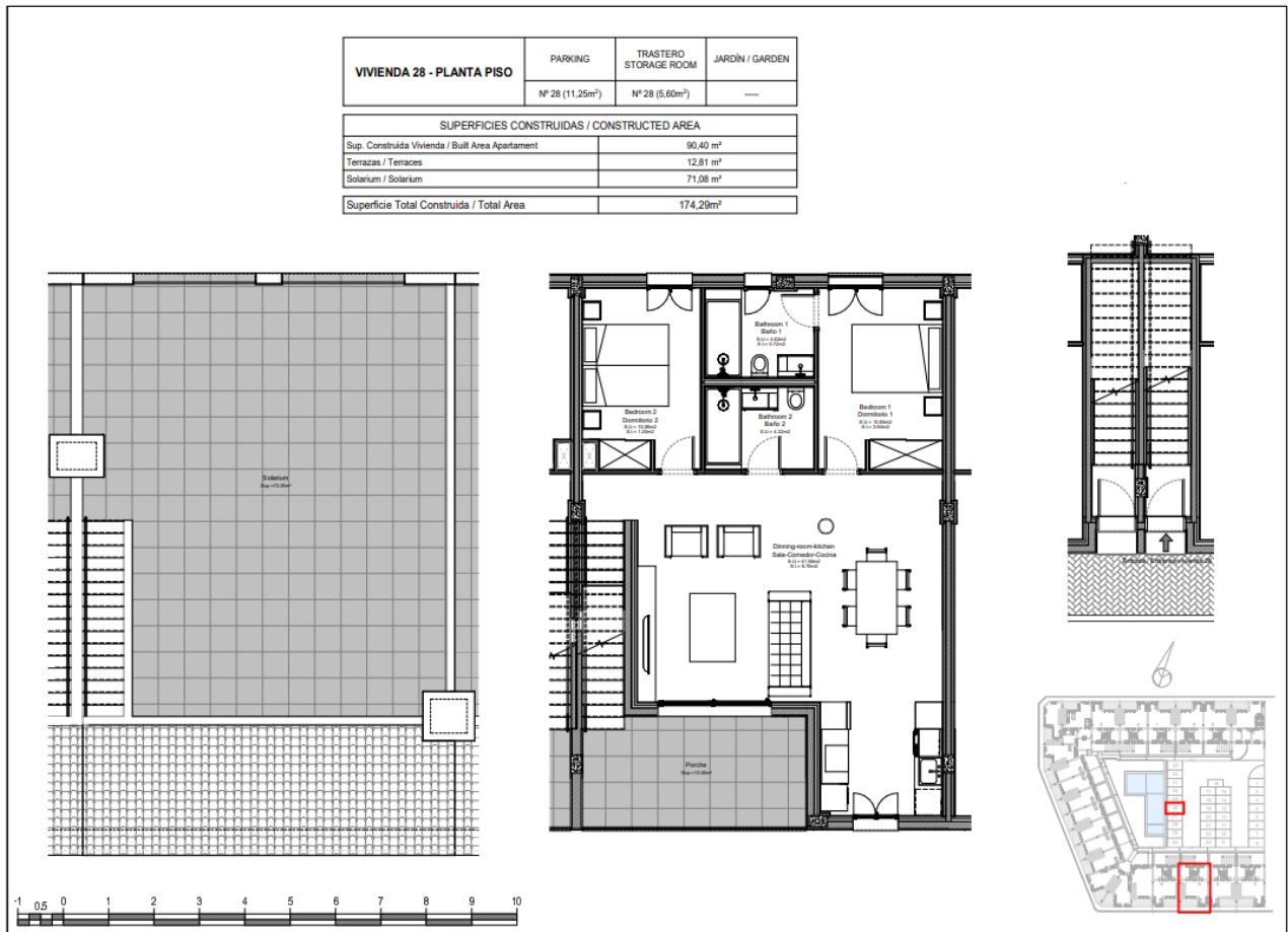
Plano B1-AT-28
